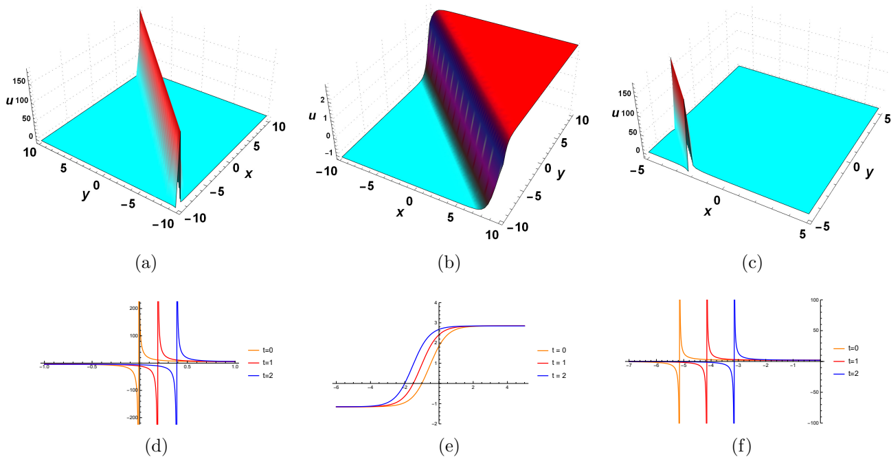
Figure 1: Graphics for the solutions (12), (13), and (15) as in (a) (b) and (c) respectively, with their 2D plots in (d), (e), and (f), having parameters : (a) t = 0, j = 1, s = -5, k = 5, \lambda = .1, J_0 = 1 ; (b) t = 0, j = 1, s = 2, k = 2, \lambda = 1.1, J_0 = 1 ; (c) t = 0, j = 1, s = -1, k = -1, \lambda = -7, J_0 = 1 .
