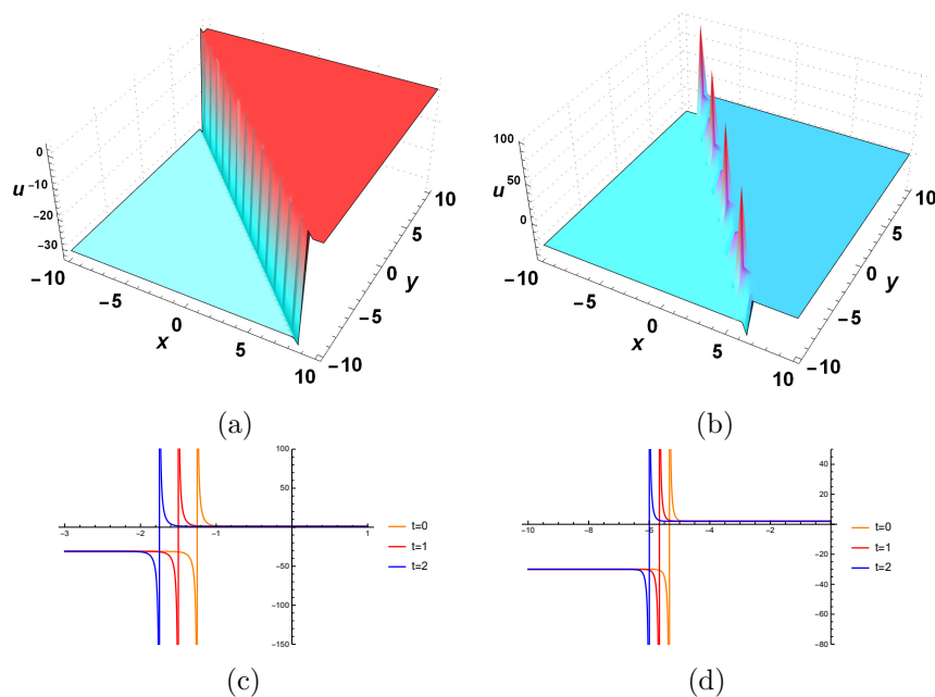
Figure 3: Graphics for the solutions (23), and (24) as in (a) and (b) respectively, with their 2D plots in (c) and (d), having parameters : (a) t = 0, j = 1, s = 4, k = 4, \lambda = 5, J_0 = 1 ; ; (b) t = 0, j = 1, s = 4, k = 3, \lambda = 4, J_0 = 2 .
