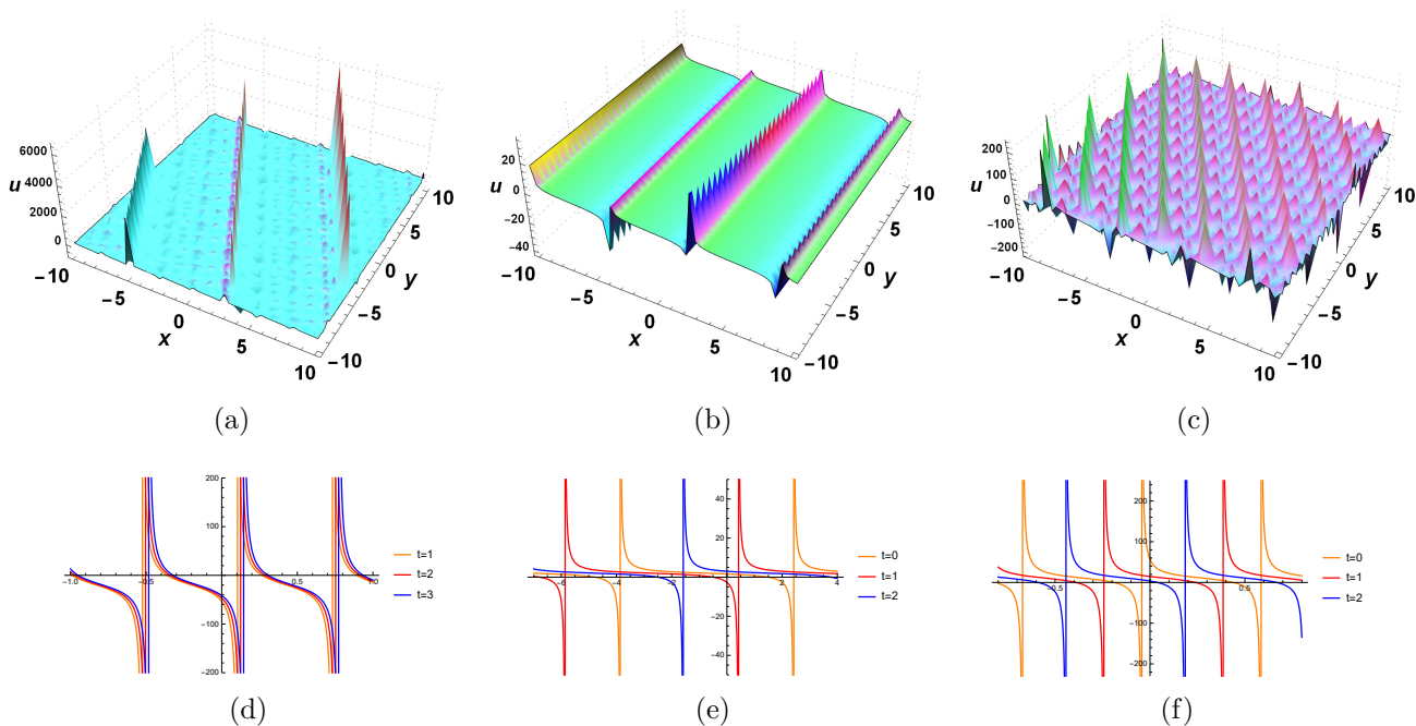
Figure 4: Graphics for the solutions (27), (28), and (30) as in (a) (b) and (c) respectively, with their 2D plots in (d), (e), and (f), having parameters : (a) t = 1, j = -.1, s = 10, k = 5, \lambda = 9, J_0 = 1 ; (b) t = 0, j = 1, s = 0.5, k = .001, \lambda = 9, J_0 = 1 ; (c) t = 0, j = 1, s = 5, k = 3, \lambda = 1, J_0 = 1 .
