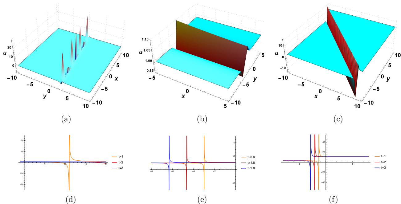
Figure 2: Graphics for the solutions (18), (19), and (20) as in (a) (b) and (c) respectively, with their 2D plots in (d), (e), and (f), having parameters : (a) t = 1, j = 1, s = -.1, k = -.8, \lambda = .1, J_0 = 1 ; ; (b) t = .8, j = 2, s = .02, k = 1.2, \lambda = 2, J_0 = 1 ; ; (c) t = 1, j = 3, s = 4, k = 4, \lambda = 2.3, J_0 = 3 .
